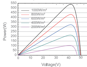
Power-Voltage Curve JAM72S30-540/MR/1500V
